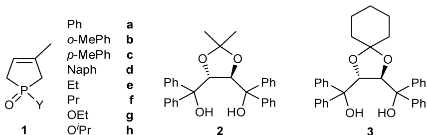
FIGURE 1 Racemic phospholene oxides ( 1 ) and the resolving agents ( 2 and 3 ).
